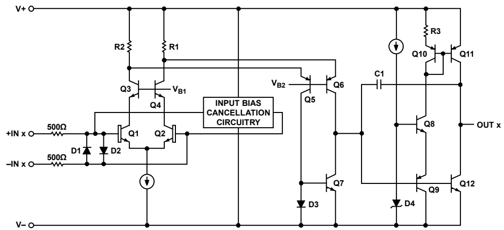
Figure 58. Simplified Schematic
